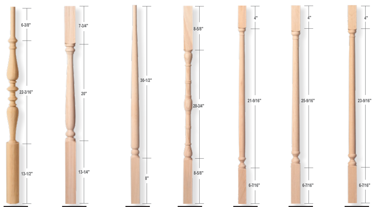
B-8 2-3/4" x 42" B-20 2-1/4" x 41" B-21 1-3/4" x 39" B-22 1-3/4" x 38" B-25 1-1/2" x 32" B-26 1-1/2" x 36" B-27 1-1/2" x 34"
