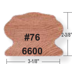
Raleigh Bending Rail 6600 B 10 Pieces
