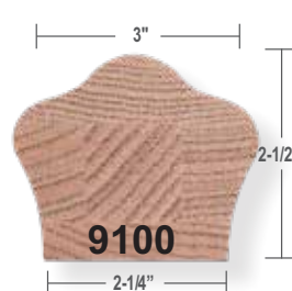
Bending Rail & Fittings Available
