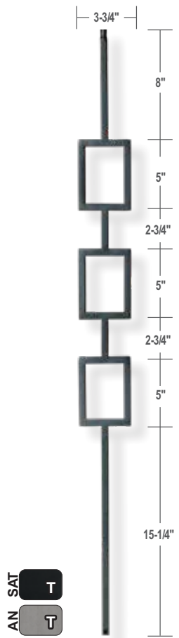
T-CS 16.6.5 Ends: 1/2" Ht: 44"
