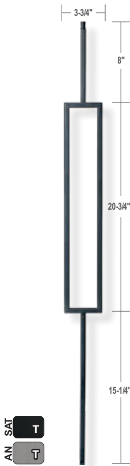
T-CS 16.6.3 Ends: 1/2" Ht: 44"
