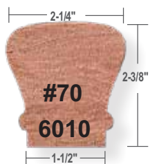
Traditional Bending Rail 6010 B 7 Pieces
