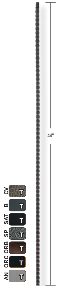
CS 16.1.7 Ends: 9/16" Square Ht: 44"
