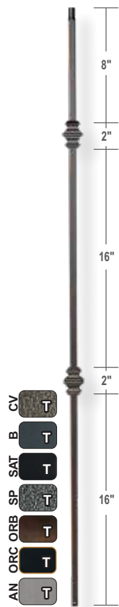
CS 16.1.35 Ends: 1/2" Ht: 44"
