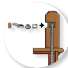
1108 Newel Anchor 11" Lag Bolt | 1 Curved Washer 1 Nut | 1-1/2" Oak and Poplar Tapered Plugs
