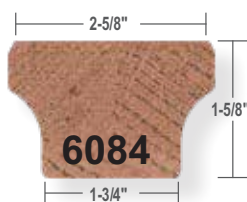
Modern Bending Rail & Fittings Available
